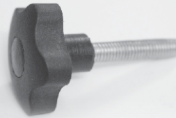
Polymide knob Dia 40 M8 X 40 RHA-128
