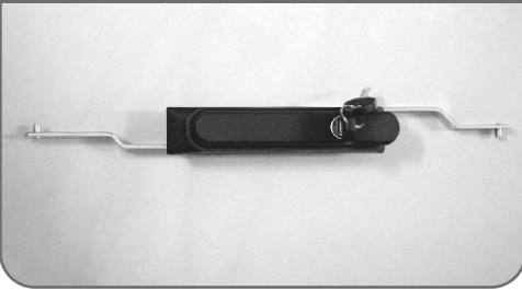
3 point Lock Swing Handle with flat Rod RCL-170
