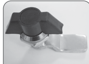
Polymide wing knob 25 mm Cut out 20 X 22 RCL-169
